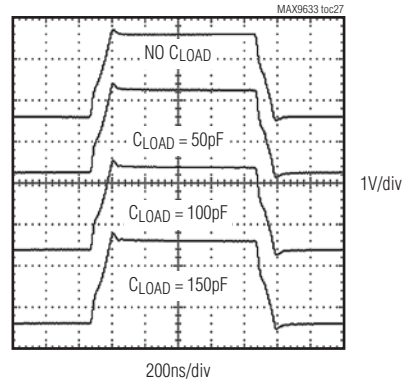
2V STEP RESPONSE WITH C_LOAD
