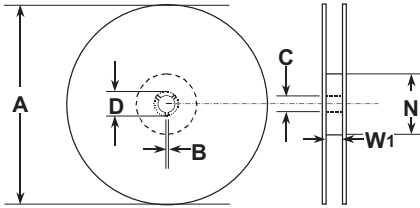
Reel Dimension
