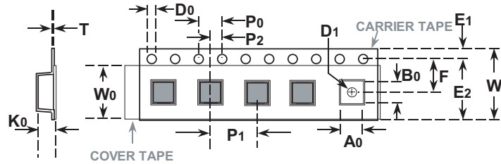
Tape Dimension Items
