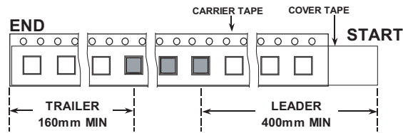
Tape Leader and Trailer Dimensions
