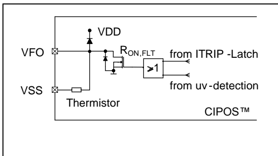
Figure 5: Internal circuit at pin VFO
