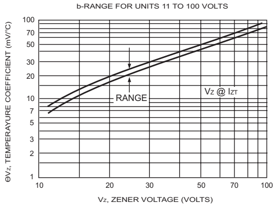
FIG.8- TEMPERATURE COEFFICIENTS
