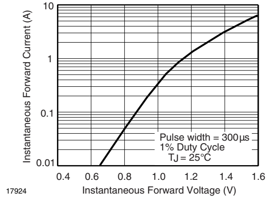
Fig. 4 - Typical Instantaneous Forward Characteristics for SML4763
