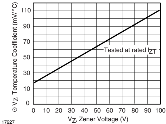
Fig. 3 - Typical Temperature Coefficients
