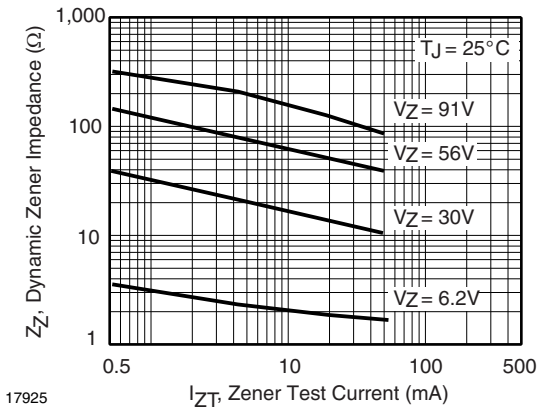
Fig. 2 - Typical Zener Impedance
