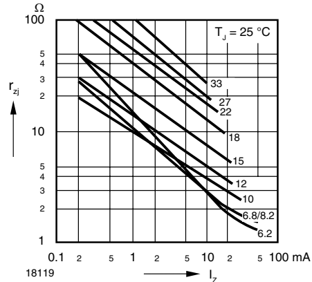
Figure 6. Dynamic Resistance vs. Zener Current
