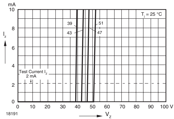
Figure 18. Breakdown Characteristics
