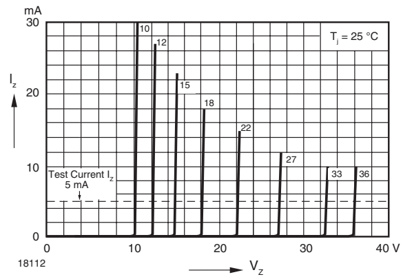
Figure 17. Breakdown Characteristics
