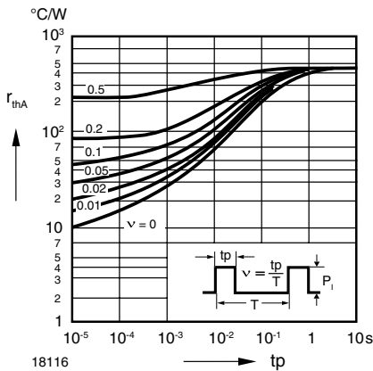
Figure 3. Pulse Thermal Resistance vs. Pulse Duration
