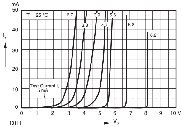
Figure 16. Breakdown Characteristics
