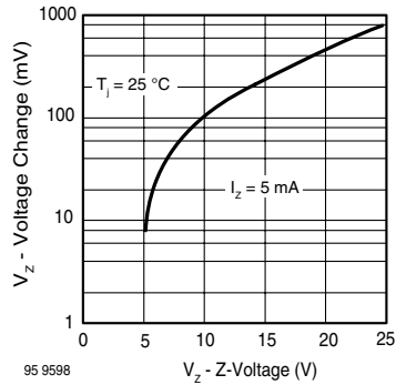
Figure 3. Typical Change of Working Voltage under Operating Conditions at T_{amb} = 25\text{ °C}
