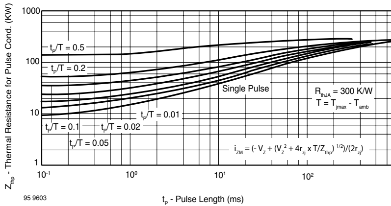
Figure 11. Thermal Response
