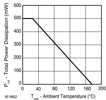
Figure 2. Total Power Dissipation vs. Ambient Temperature
