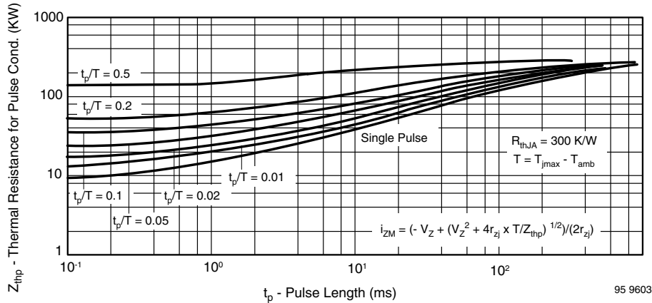
Figure 13. Thermal Response
