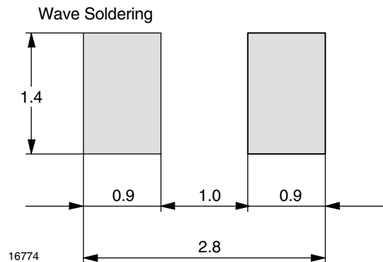
Figure 12. Recommended Foot Pads (in mm)
