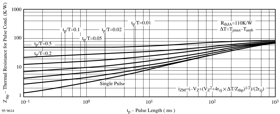
Figure 5. Thermal Response
