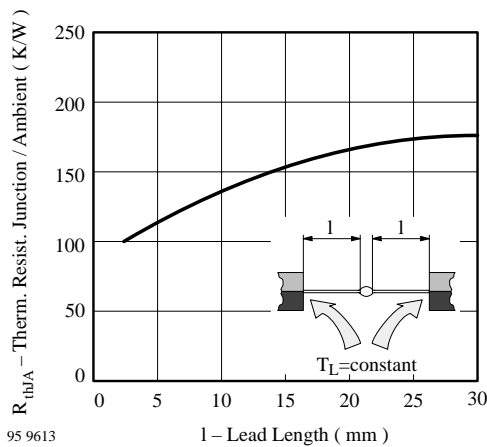
Figure 2. Thermal Resistance vs. Lead Length
