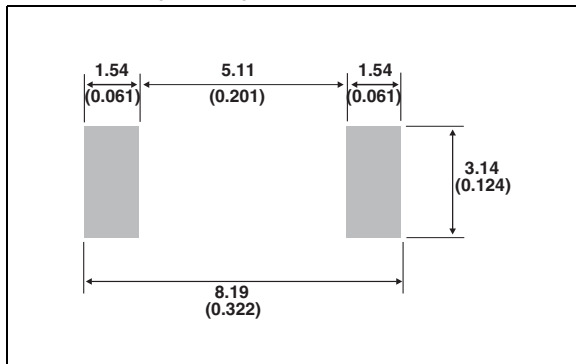
Figure 13. SMC footprint dimensions in mm (inches)
