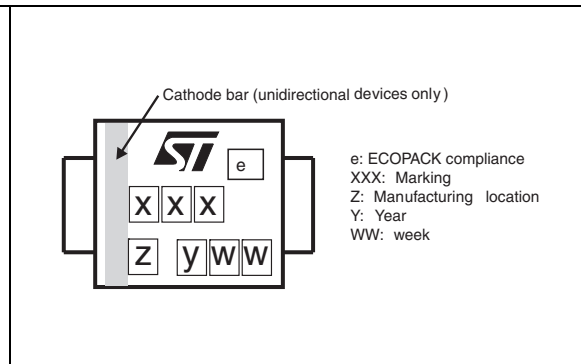
Figure 14. Marking layout (1)
