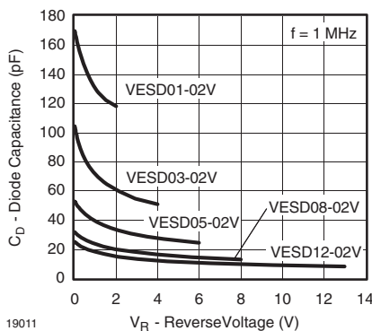
Figure 2. Typ. Diode Capacitance vs. Reverse Voltage
