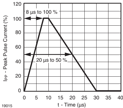
Figure 1. Pulse Waveform 8/20 \mu\text{s} acc. IEC 61000 - 4 - 5
