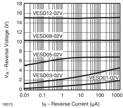
Figure 5. Reverse Voltage vs. Reverse Current
