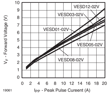
Figure 6. Typical Forward Voltage vs. Peak Pulse Current
