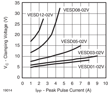
Figure 3. Clamping Voltage vs. Peak Pulse Current
