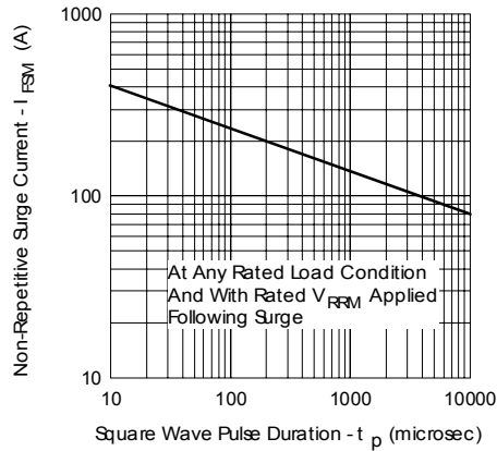
Fig. 7 - Max. Non-Repeticitive Surge Current (Per Leg)
