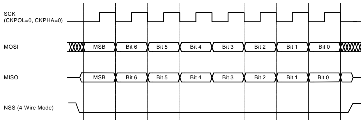
Figure 14.2. Data/Clock Timing
