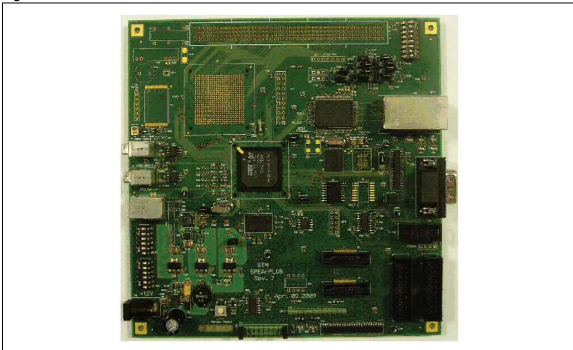
Figure 1. EVALSPEAr600 evaluation board
