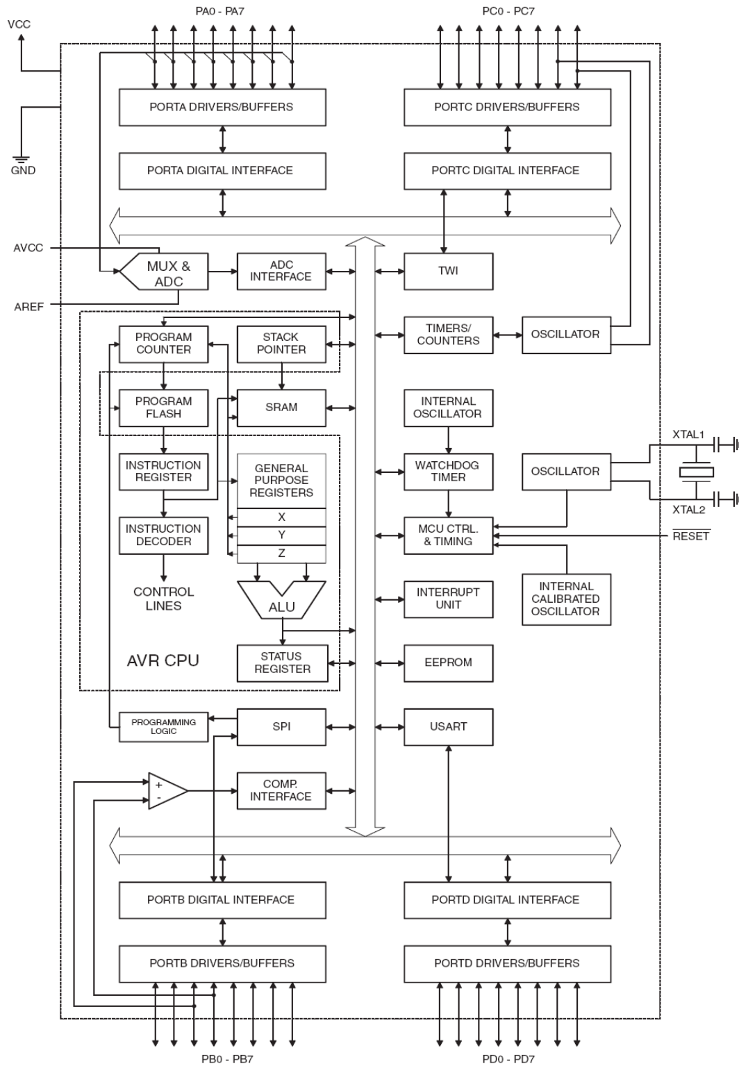
Figure 2. Block Diagram
