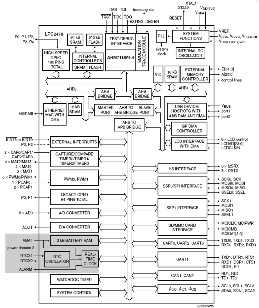
Fig 1. LPC2478 block diagram
