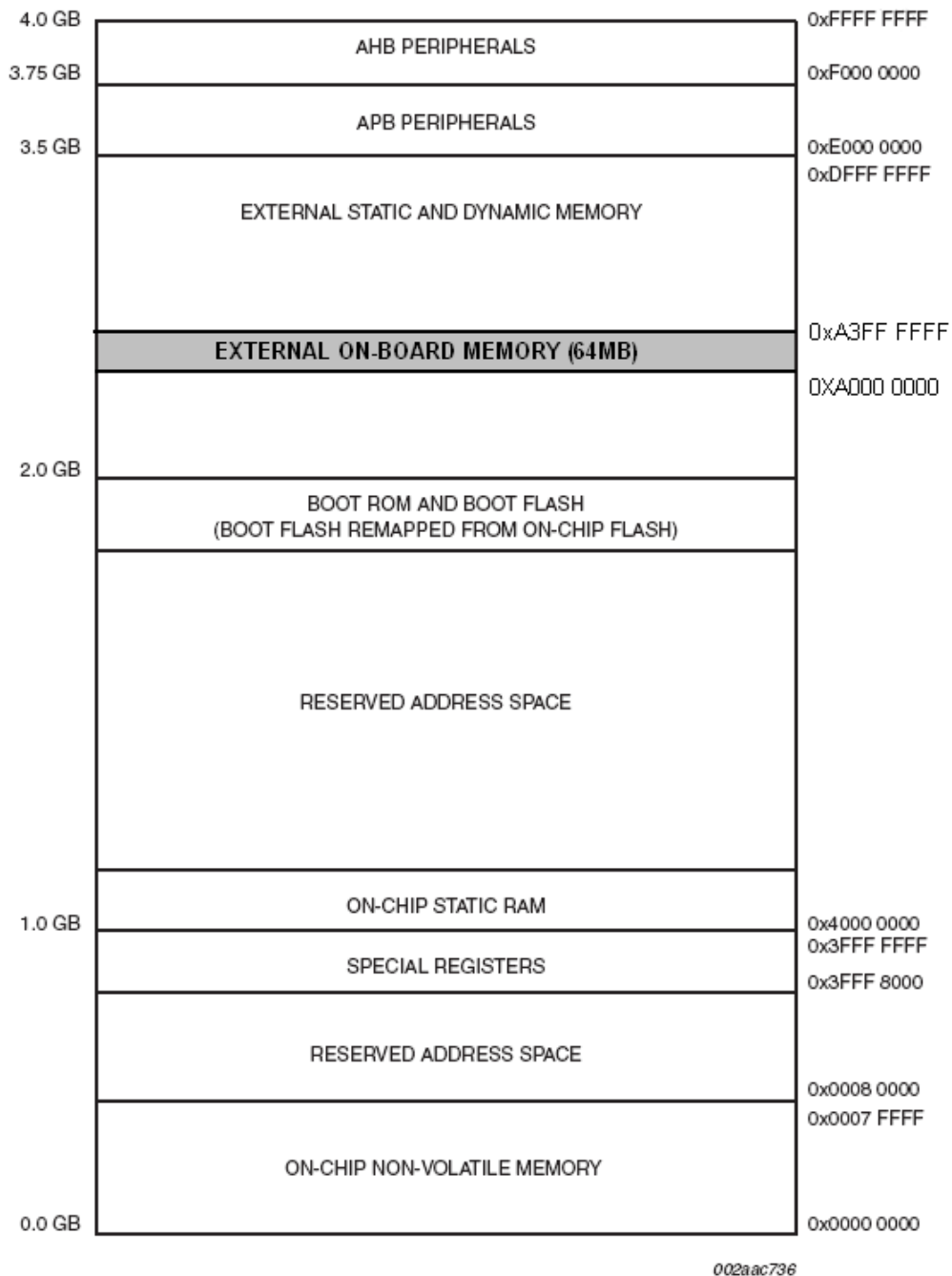
Fig 4. LPC2478 memory map
