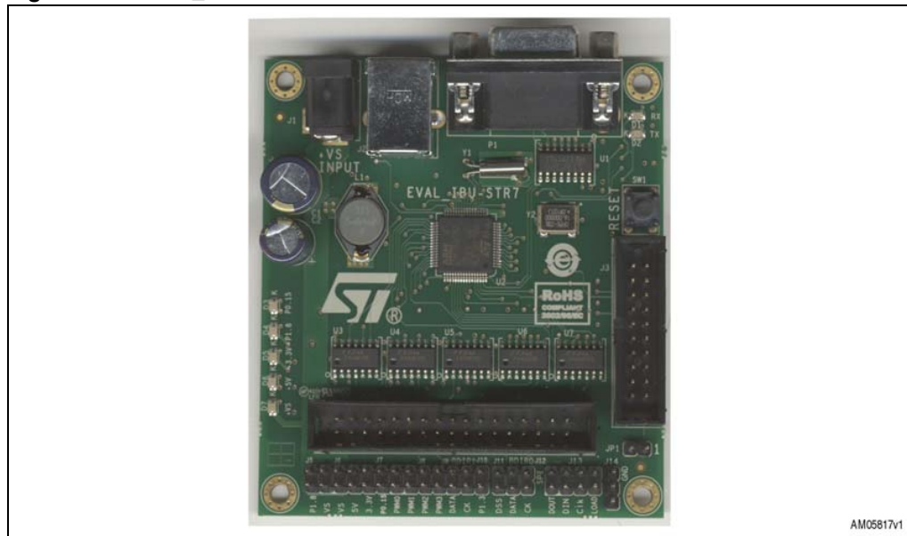
Figure 5. EVAL_IBU-STR7 board
