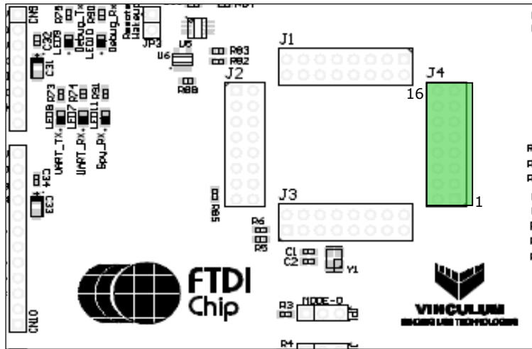
Figure 5.25 VNC2 Daughterboard Connector J4.
