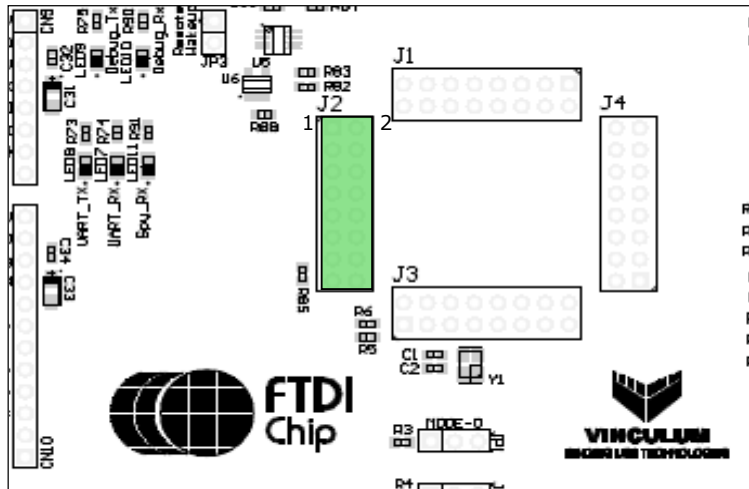
Figure 5.23 VNC2 Daughterboard Connector J2.
