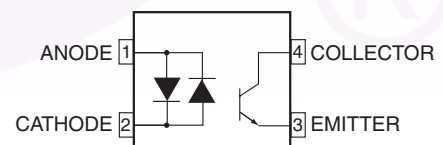
Equivalent Circuit FODM2705
