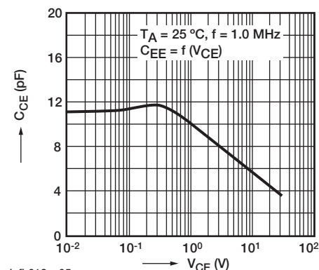
Fig. 7 - Transistor Capacitance
