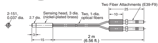
E32-D22R Free-cut
