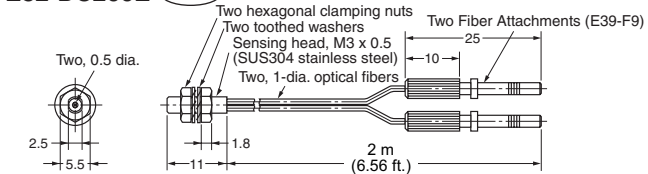
E32-DC200E Free-cut
