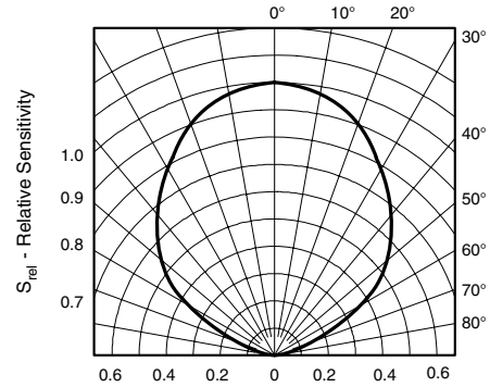
Figure 6. Relative Radiant Sensitivity vs. Angular Displacement
