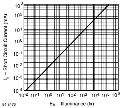
Figure 3. Short Circuit Current vs. Illuminance
