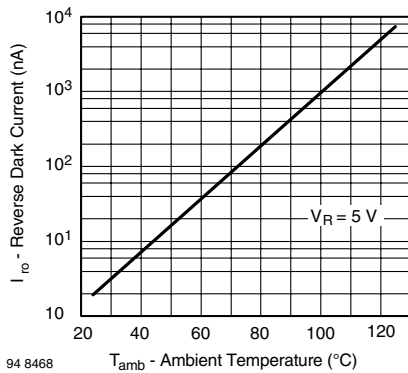
Figure 1. Reverse Dark Current vs. Ambient Temperature
