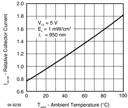
Figure 2. Relative Collector Current vs. Ambient Temperature
