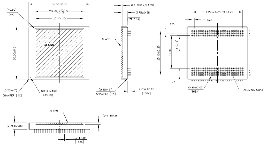
Figure 35. Package Outline Drawing for the LUPA 1300-2 168-Pin \mu PGA
