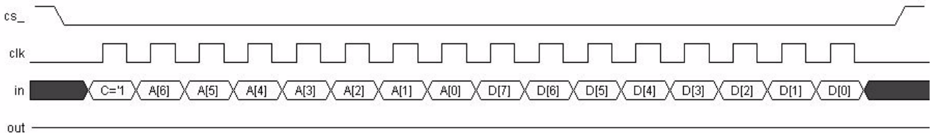
Figure 9. Write Access (C='1')
