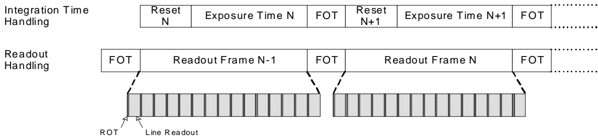
Figure 13. Global Readout Timing (Parallel)
