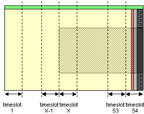
Figure 19. Single Window Containing Timeslot 54
