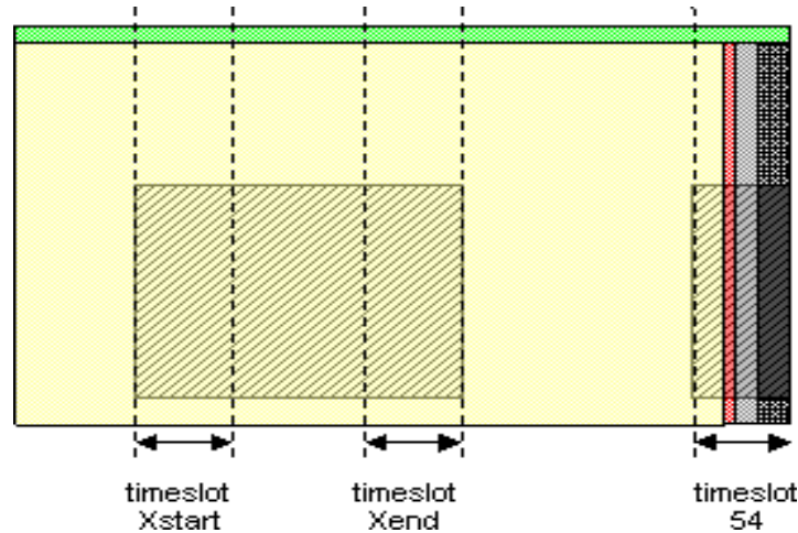
Figure 21. Single Window Not Containing Timeslot 54
