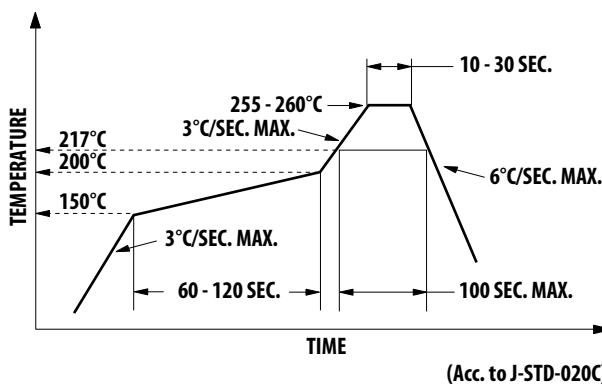
Figure 20. Recommended Reflow Soldering Profile.
