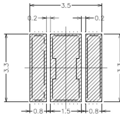
Soldering patterns
