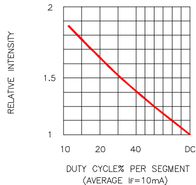
Fig.4 LUMINOUS INTENSITY VS. DUTY CYCLE
