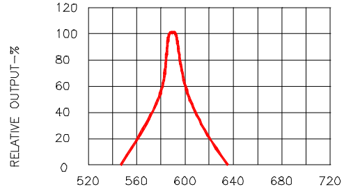
Fig.2 SPECTRAL RESPONSE
