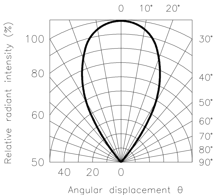
Radiation Diagram
