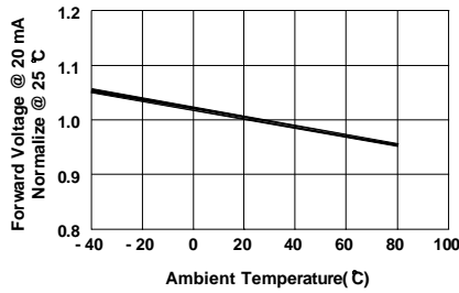
Fig 3. Forward Voltage vs. Temperature
