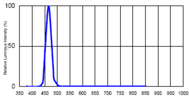
Relative Luminous Intensity vs. Wavelength
