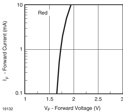
Figure 15. Forward Current vs. Forward Voltage
