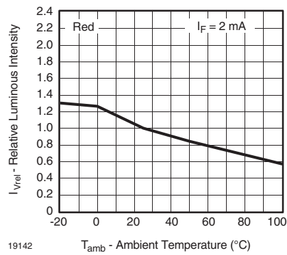
Figure 18. Relative Luminous Intensity vs. Amb. Temperature
