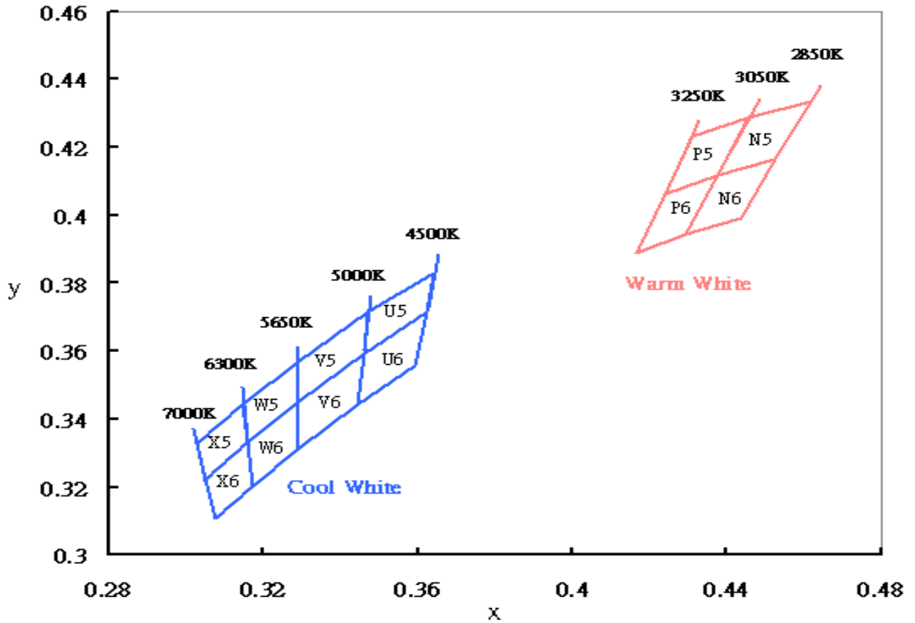
The C.I.E. 1931 Chromaticity Diagram
