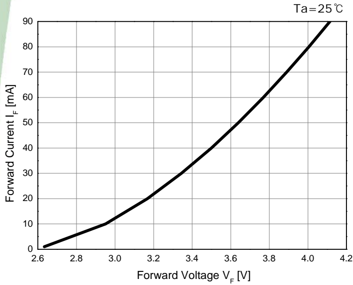
Forward Voltage vs. Forward Current (Per die)
