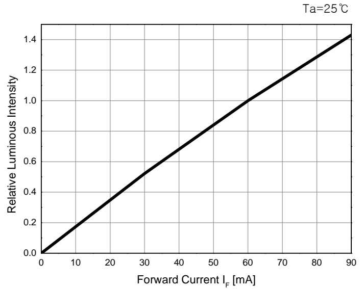
Forward Current vs. Relative Luminous Intensity
