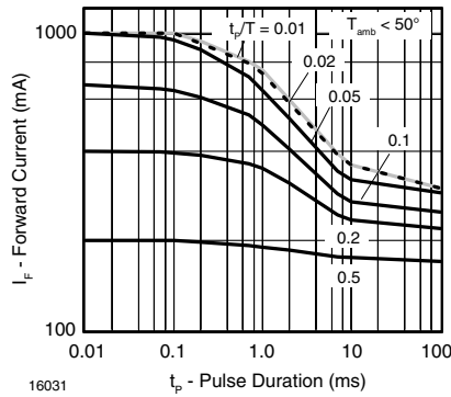
Figure 3. Pulse Forward Current vs. Pulse Duration
