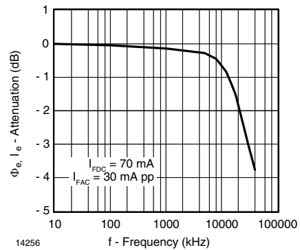
Figure 8. Attenuation vs. Frequency
