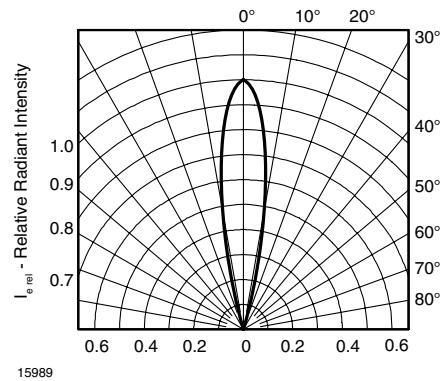
Figure 7. Relative Radiant Intensity vs. Angular Displacement
