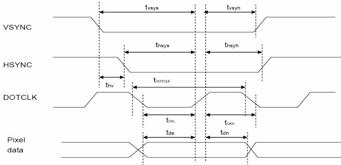
Pixel timing
