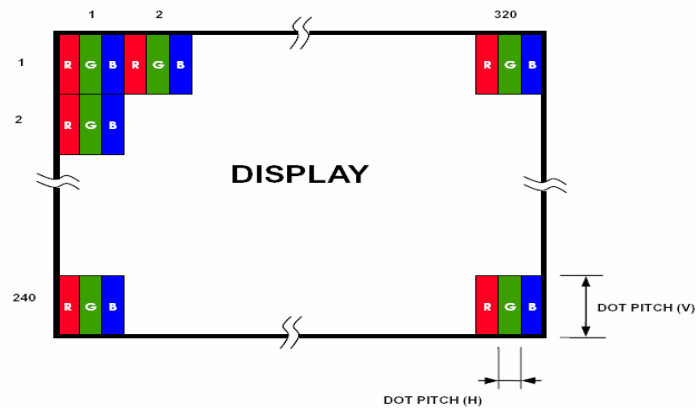
Pixel Arrangement
