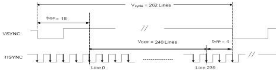
b) Vertical Data Transaction Timing
