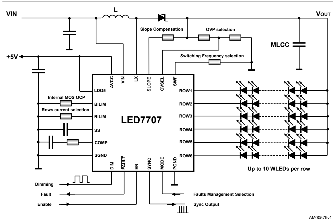
Figure 1. Application circuit
