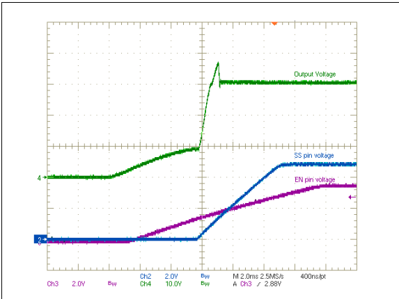
Figure 29. Soft-start waveforms (EN, SS, and V_{OUT} monitored)
