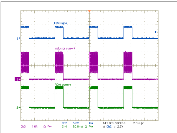
Figure 31. Dimming waveforms ( F_{DIM} = 200\text{ Hz} )
