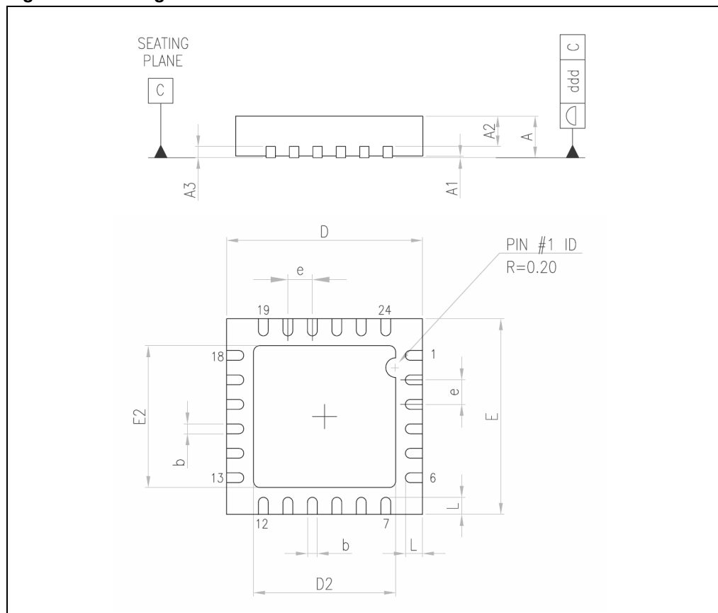
Figure 33. Package dimensions
