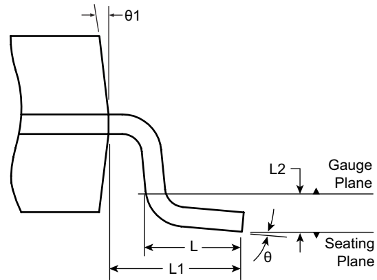
View B
