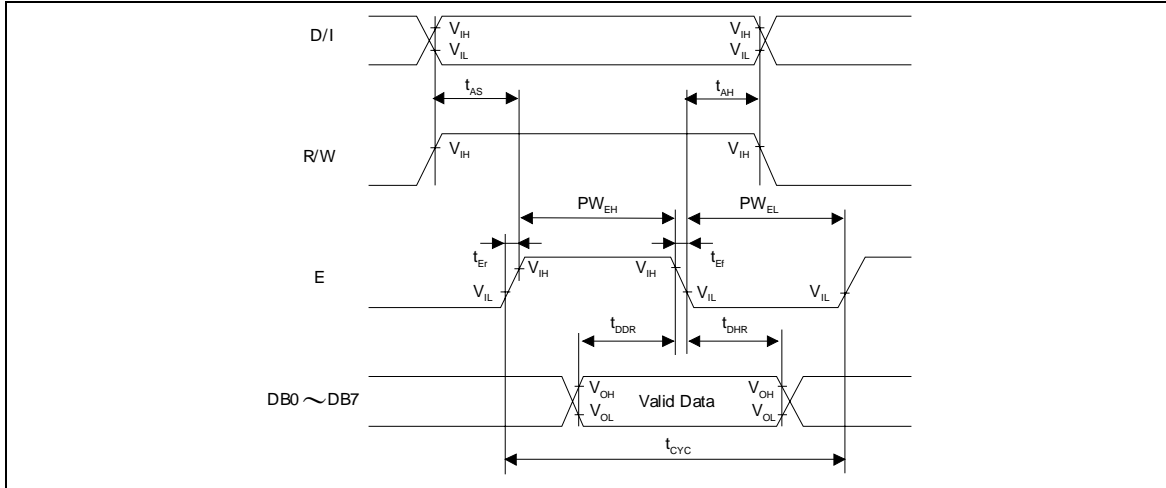
Note 2 : Read Operation Timing
