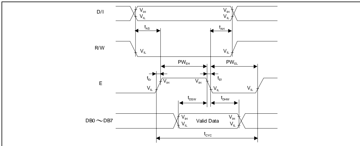
Note 1 : Write Operation Timing
