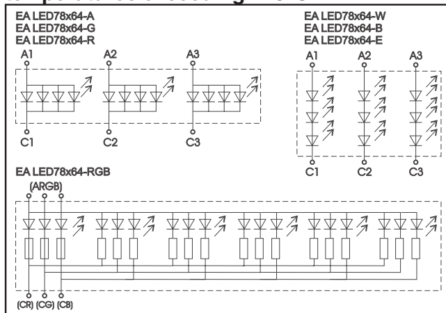
LED-Backlight schematic
