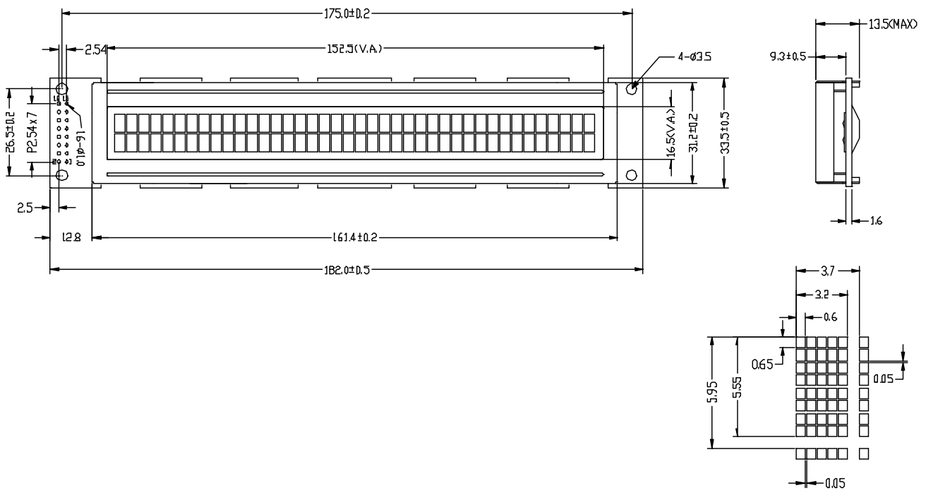
Newhaven Display NHD-0240AZ-FL-YBW
