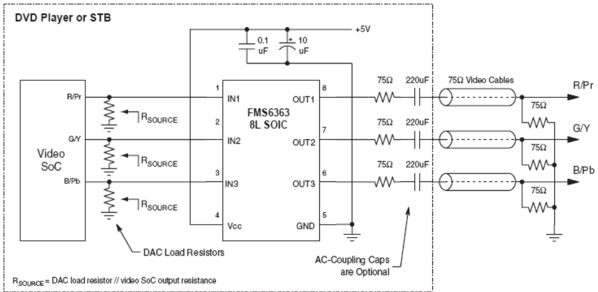
Figure 3. Typical Application
