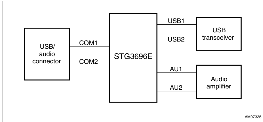
Figure 4. Application diagram
