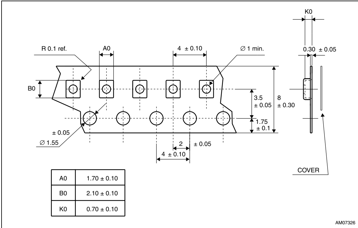
Figure 7. Carrier tape for QFN10 (1.8 x 1.4 x 0.5 mm)
