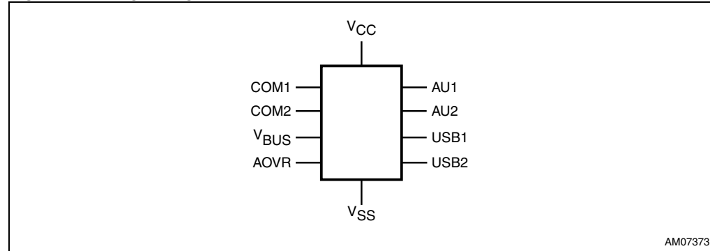
Figure 1. Logic diagram
