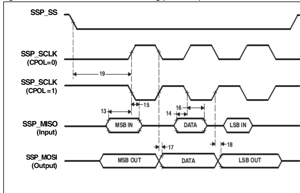
Figure 44. SPI master mode external timing (CPHA = 0)
