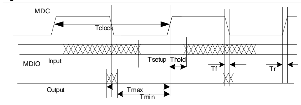
Figure 39. MDC waveforms
