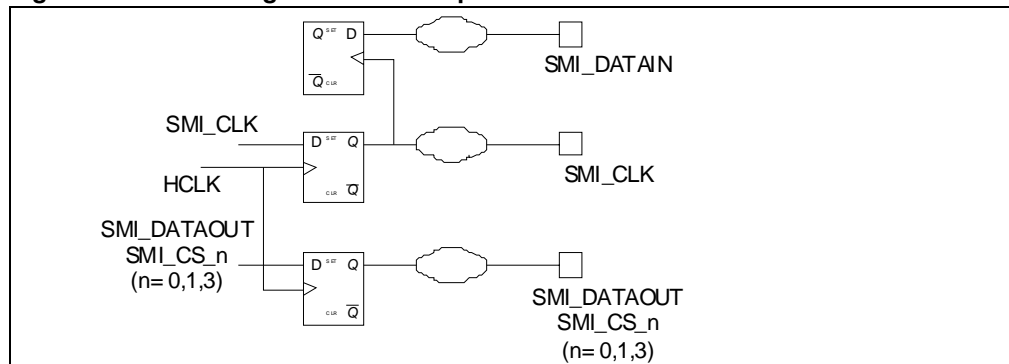
Figure 42. Block diagram of the SMI pins
