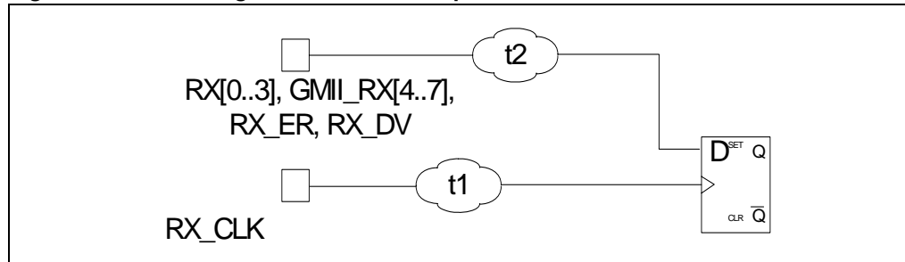
Figure 38. Block diagram of GMII-MII RX pins
