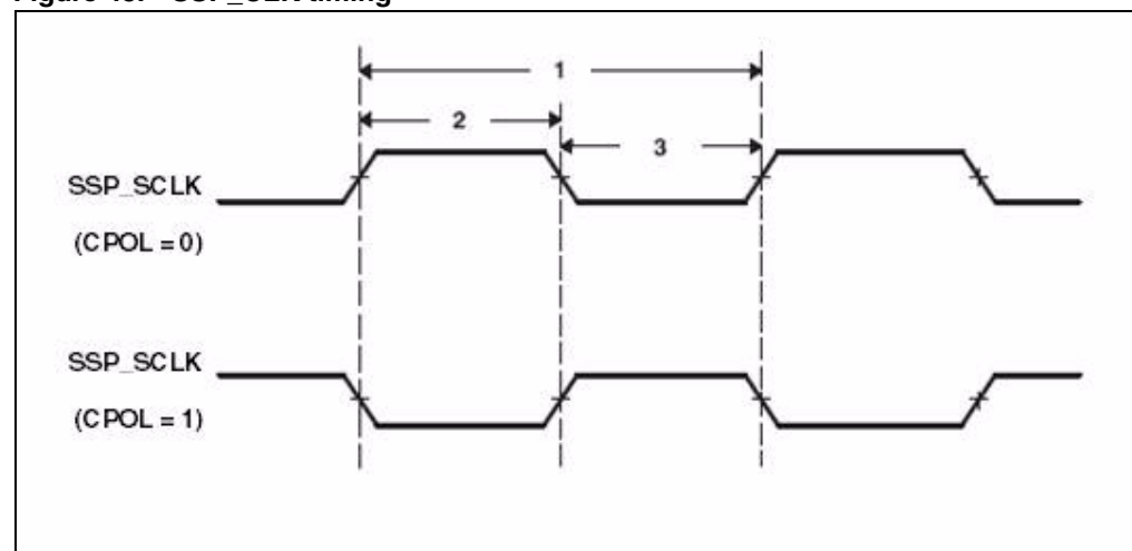
Figure 43. SSP_CLK timing
