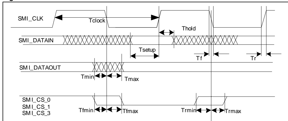
Figure 41. SMI waveforms
