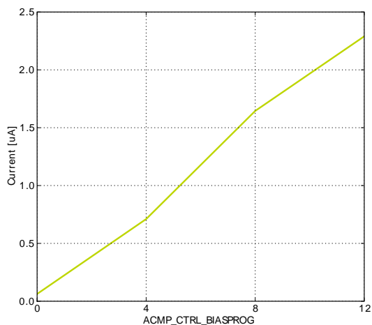
Current consumption
