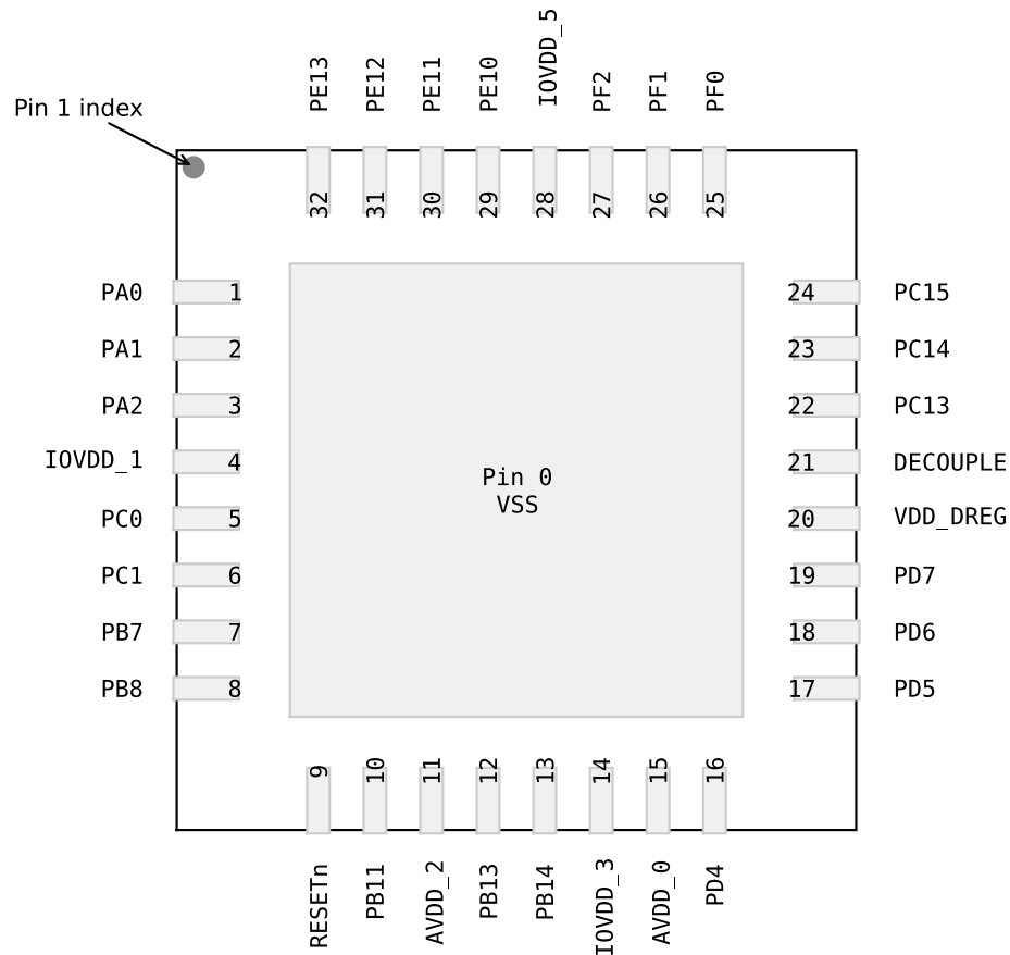
Figure 4.1. EFM32G200 Pinout (top view, not to scale)
