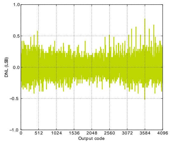
2.5V Reference
