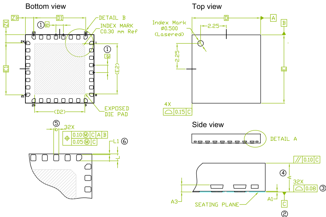
Figure 4.2. QFN32
