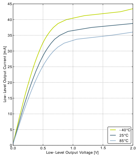
GPIO_Px_CTRL DRIVEMODE = HIGH
