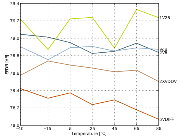
Spurious-Free Dynamic Range (SFDR)
