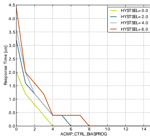
Response time
