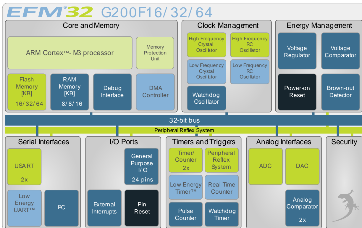
Figure 1.1. Block Diagram
