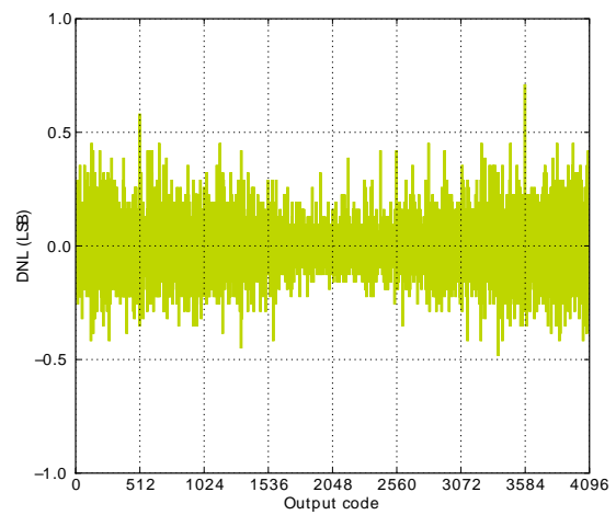
5VDIFF Reference
