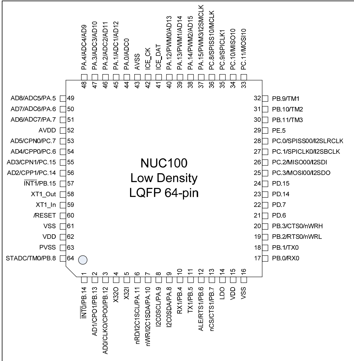
Figure 3-5 NuMicro™ NUC100 Low Density LQFP 64-pin Pin Diagram
