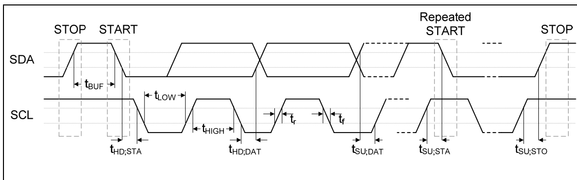
Figure 5-9 I 2 C Bus Timing
