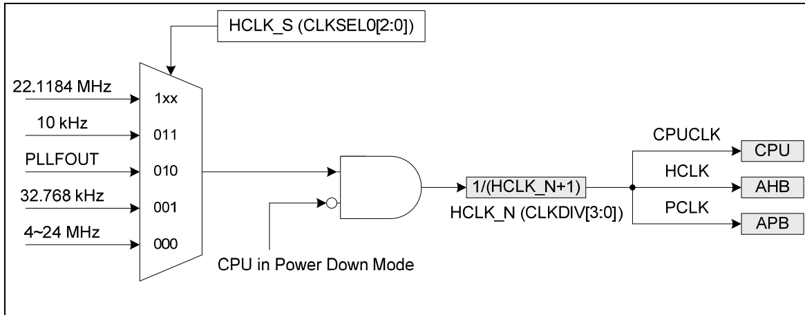
Figure 5-5 System Clock Block Diagram
