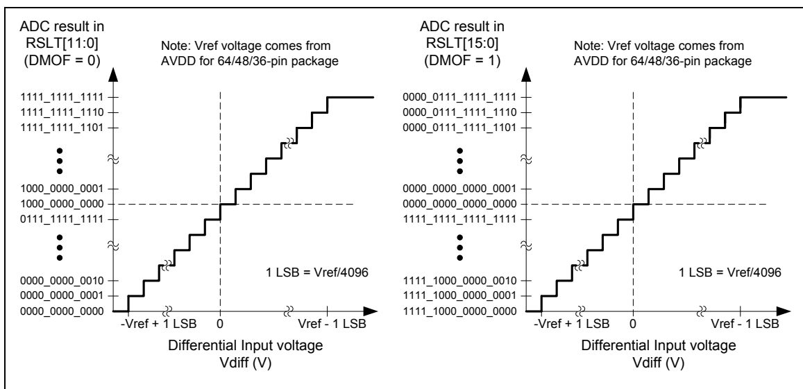
Figure 5-103 ADC differential input conversion voltage and conversion result mapping diagram
