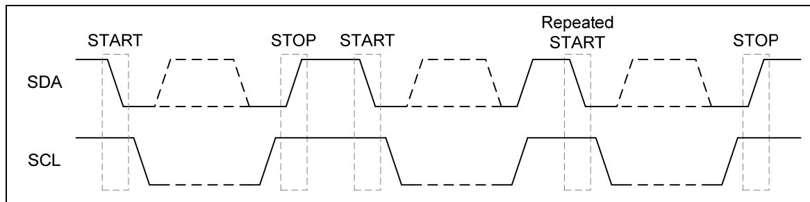
Figure 5-21 START and STOP condition
