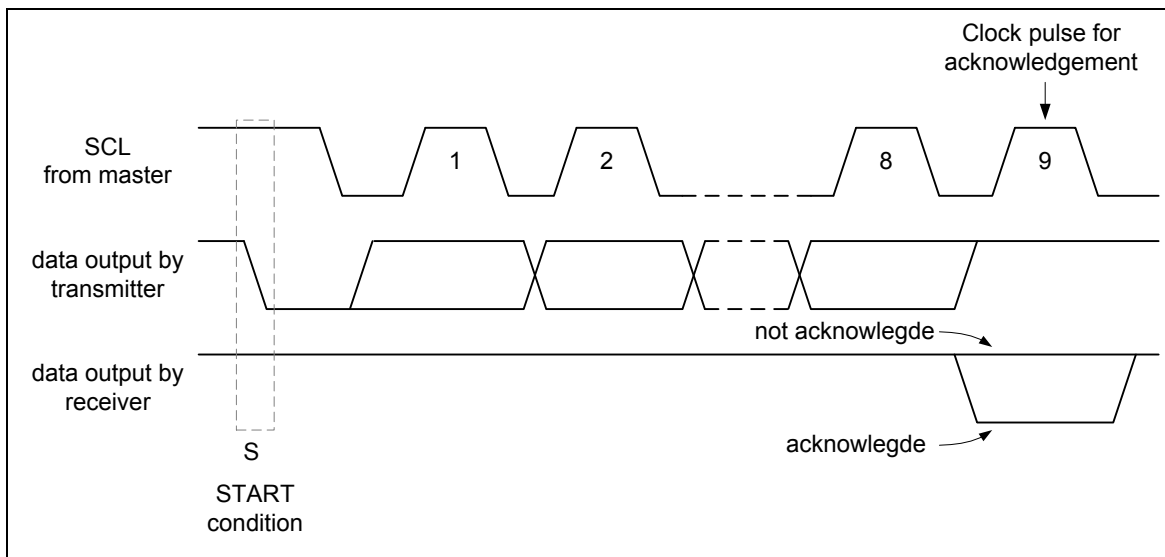
Figure 5-23 Acknowledge on the I 2 C bus
