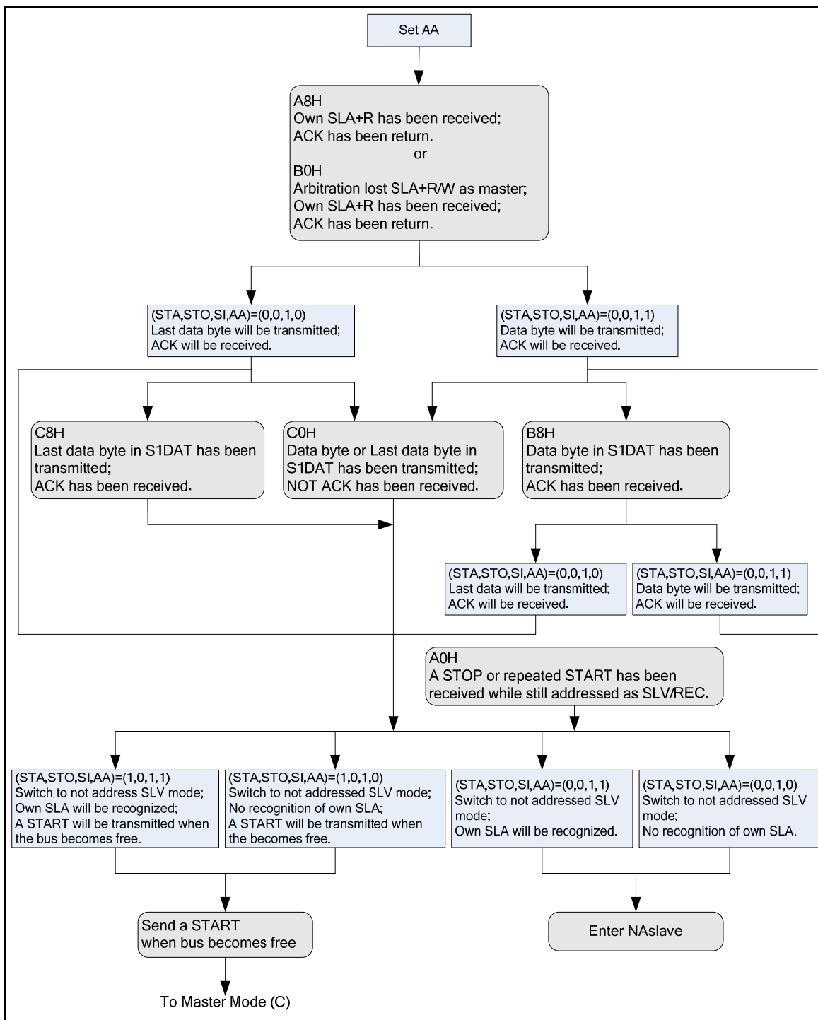
Figure 5-29 Slave Transmitter Mode
