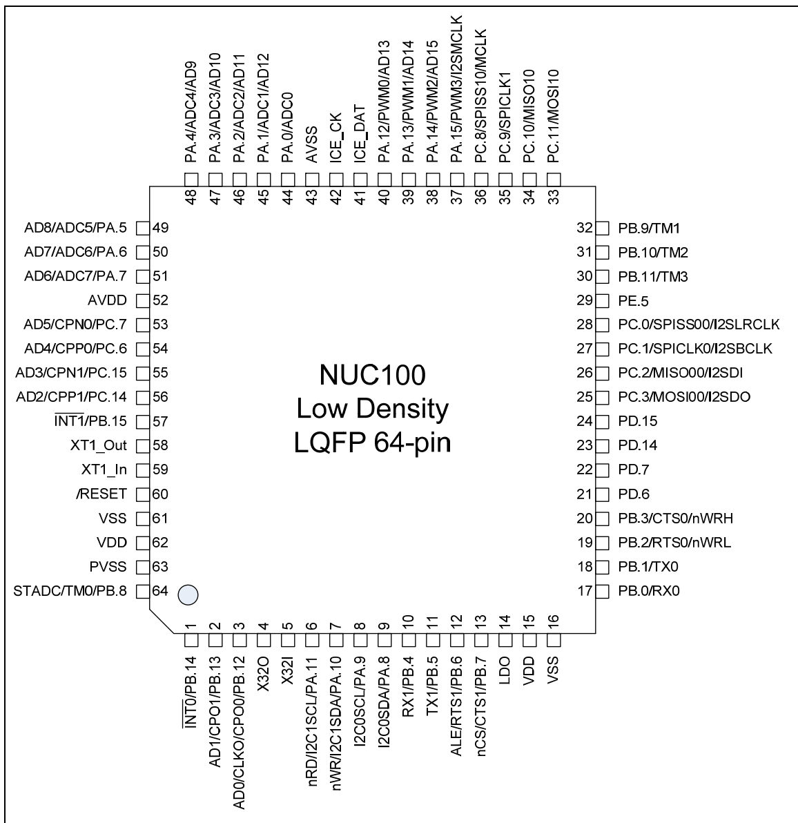
Figure 3-14 NuMicro™ NUC100 Low Density LQFP 64-pin Pin Diagram
