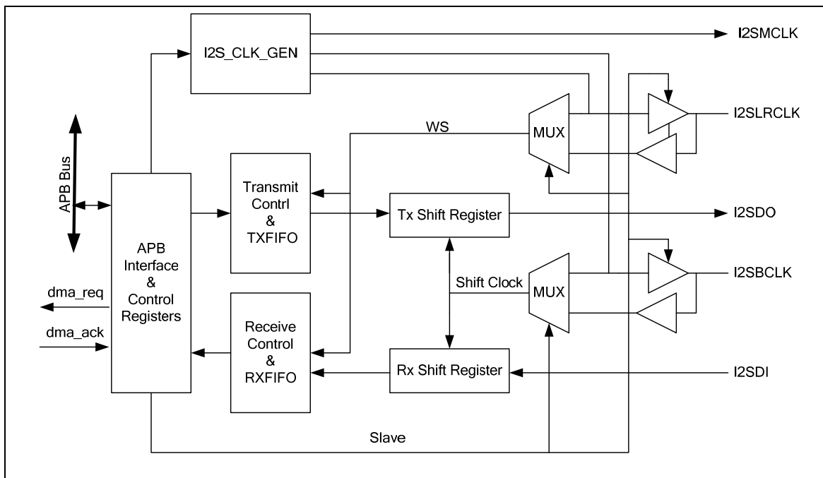
Figure 5-90 I²S Controller Block Diagram
