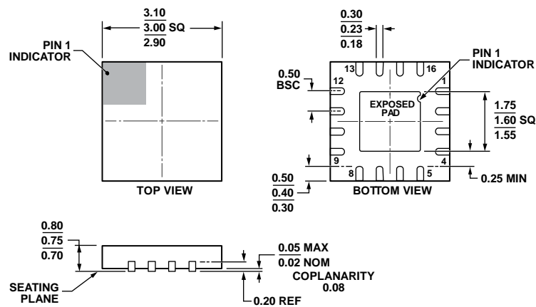
Figure 40. 16-Lead Lead Frame Chip Scale Package [LFCSP] (CP-16-22) Dimensions shown in millimeters
