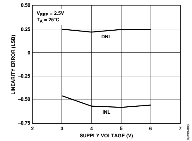
Figure 9. AD5542A Linearity Error vs. Supply Voltage
