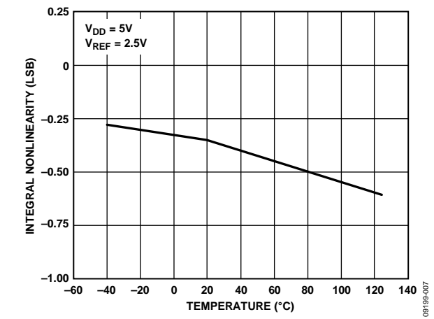
Figure 8. AD5542A Integral Nonlinearity vs. Temperature
