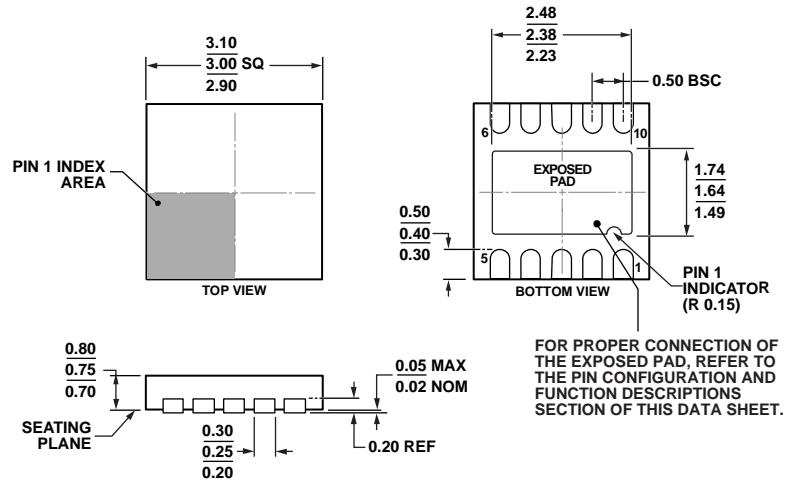
Figure 42. 10-Lead Lead Frame Chip Scale Package [LFCSP_WD] 3 mm x 3 mm Body, Very Thin, Dual Lead (CP-10-9)
