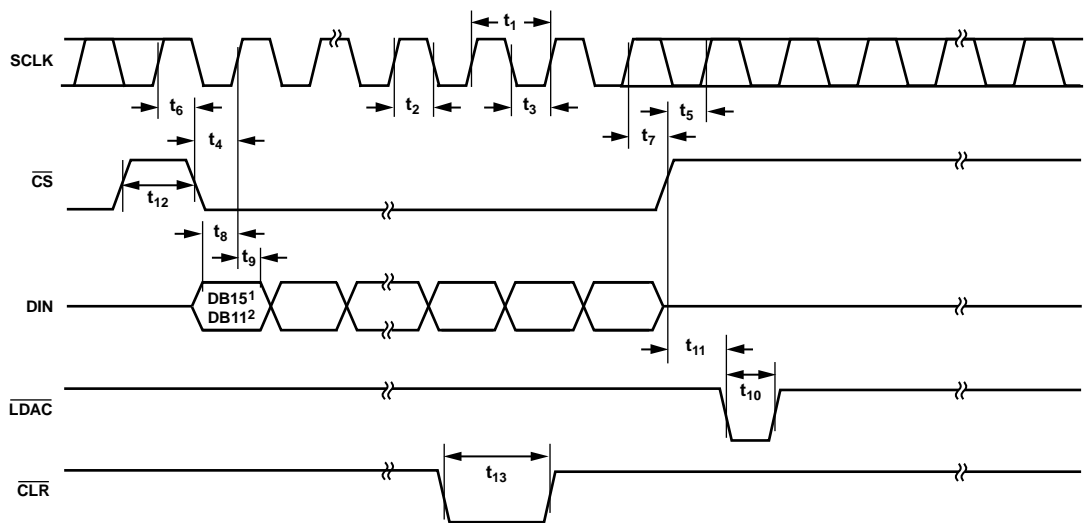
Figure 3. Timing Diagram
