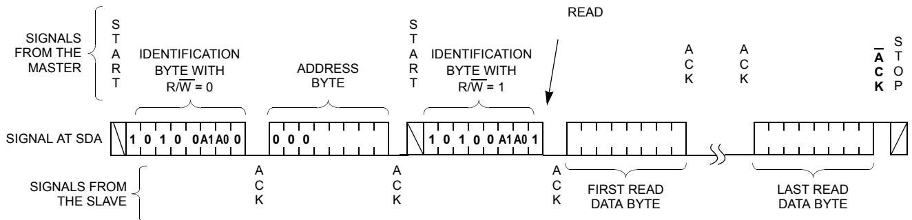
FIGURE 29. READ SEQUENCE
